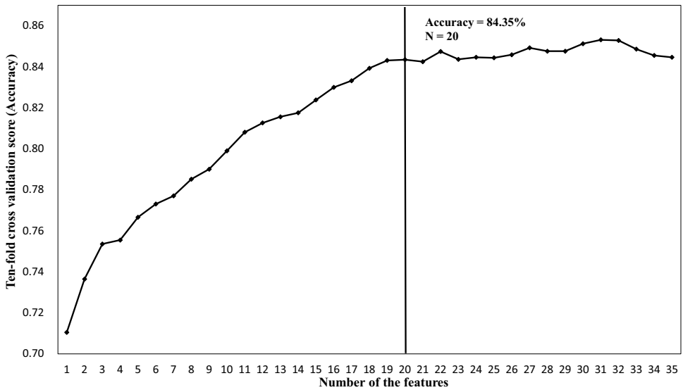
Fig. 2 The accuracy of top 35 feature sets with ten-fold cross-validation
